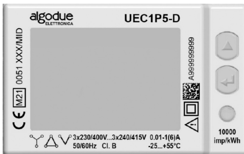
Targa / Marking plate
